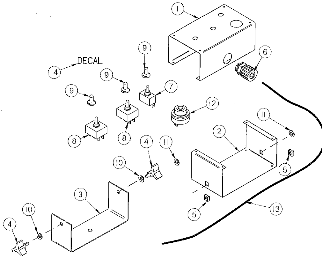
FIGURE 9 CONTROL BOX
